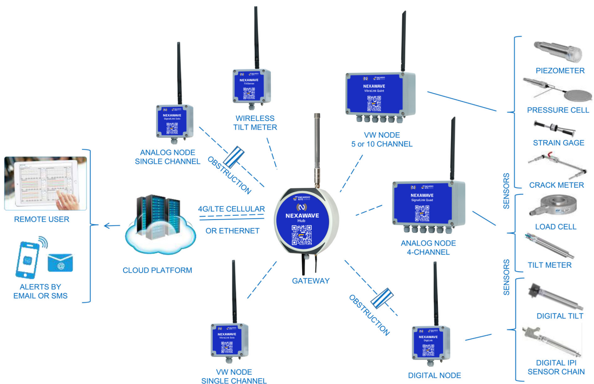
WIRELESS TILT METER WITH OTHER NODES CONNECTED TO GATEWAY IN LORA NETWORK
