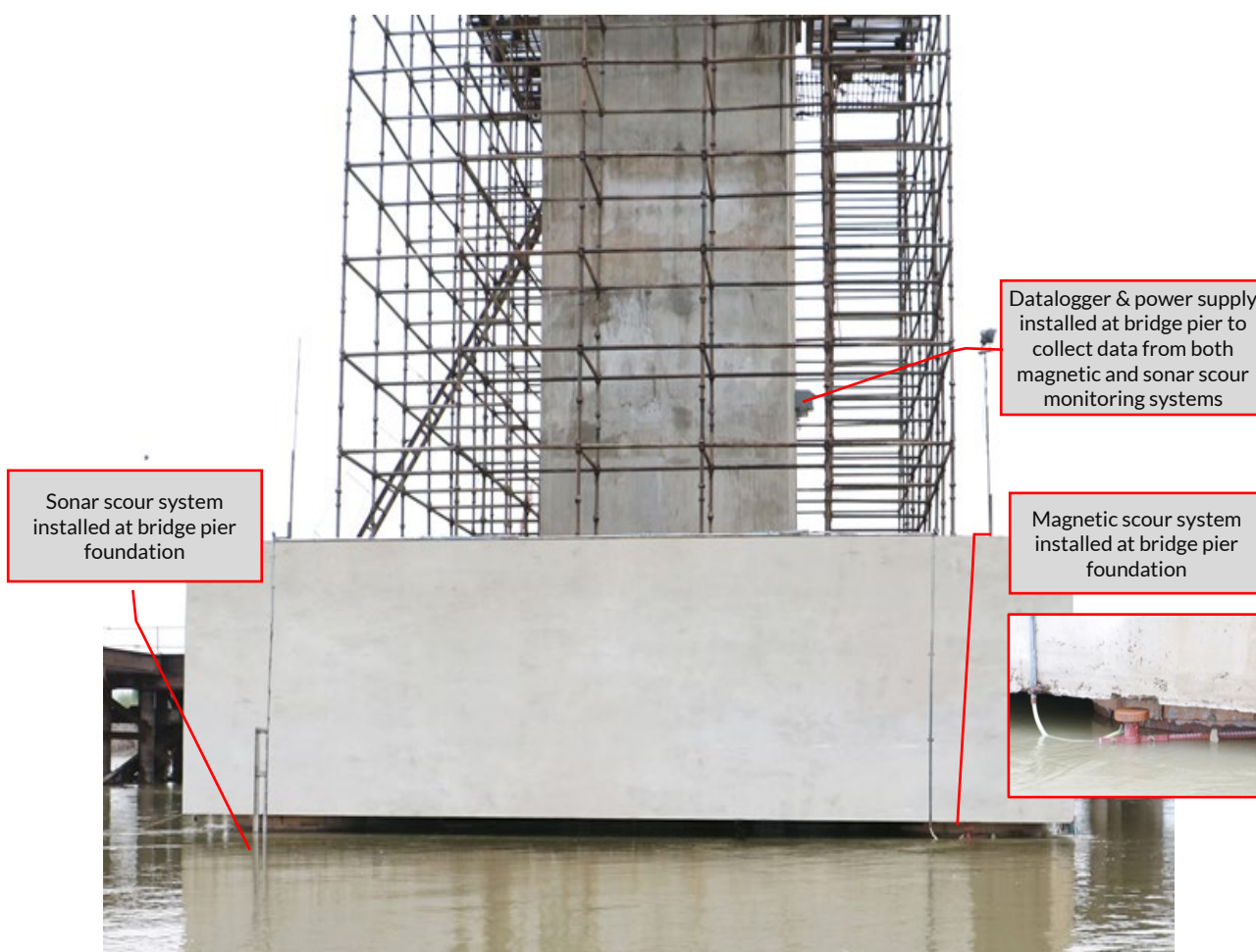
Scour monitoring system (magnetic and sonar with datalogger) installed at a bridge in India
