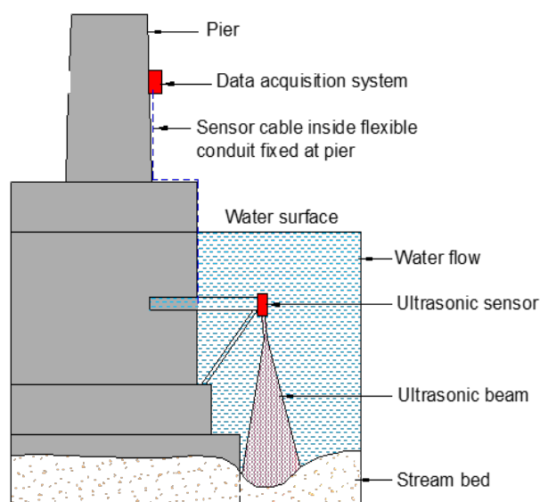
EBSM-101S Sonar scour system
