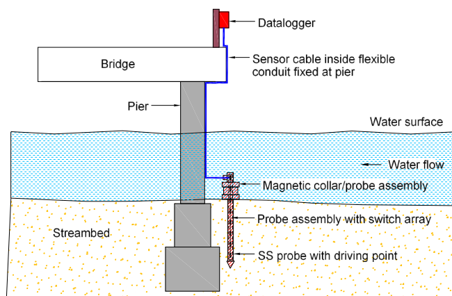
EBSM-101M Magnetic scour system
