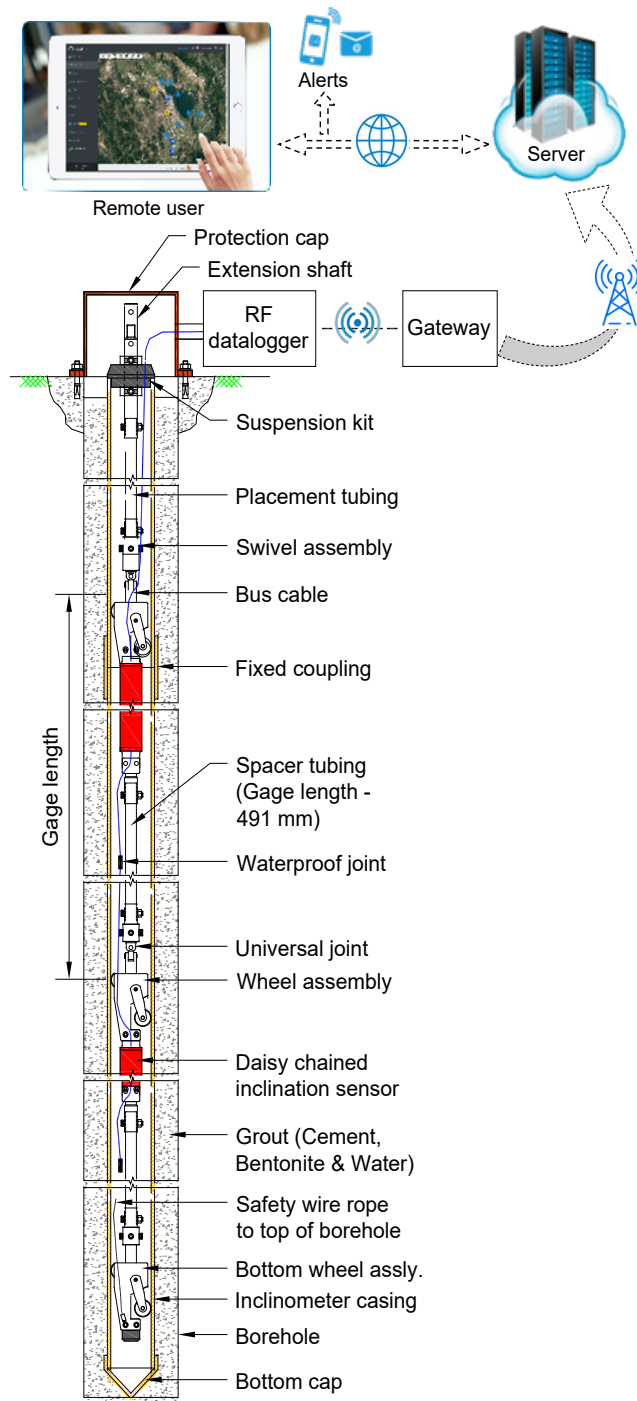
EAN-56 In-place inclinometer system with RF datalogger and gateway
